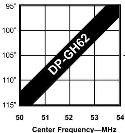
Length of Lower Radiator vs. Frequency
